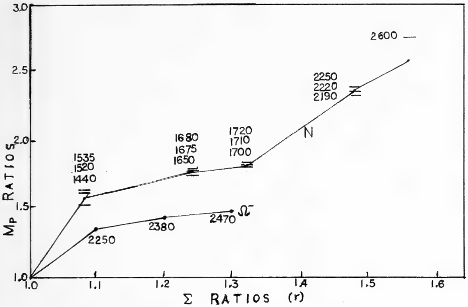
FIG. C1. Ratios of particle to reference masses vs ratios ( r_{0,1,2,3} ) of sums of component masses to reference sum for Example 2 (four Omega minus particles) and Example 3 (fourteen neutral Nucleons) of Appendix C.
